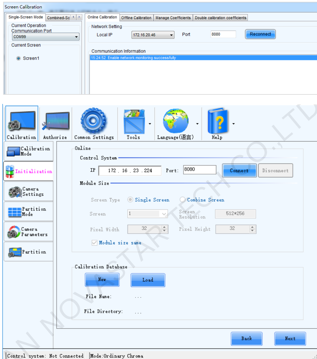
Figure 2-2 Initialization
