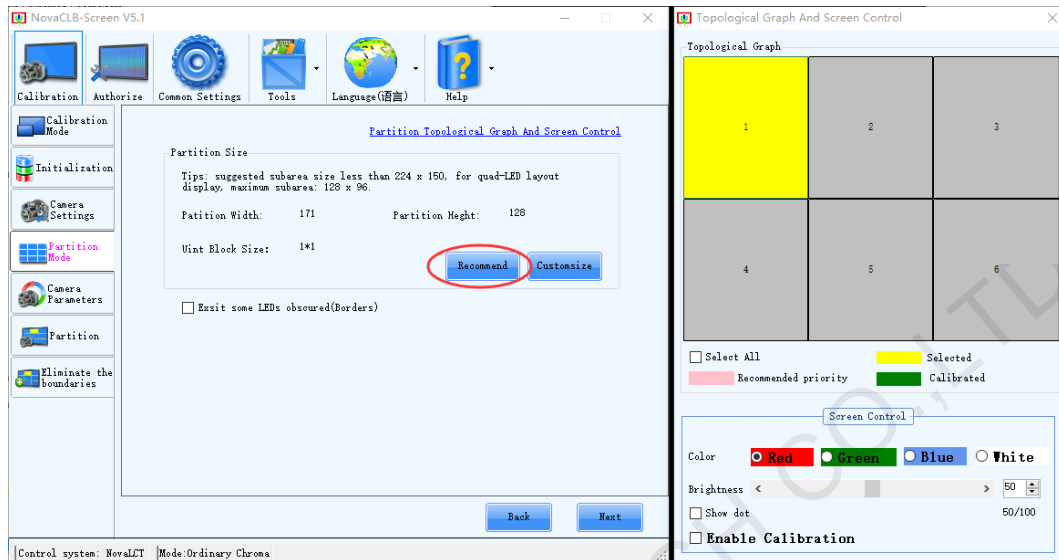
Figure 2-3 Partition Mode
