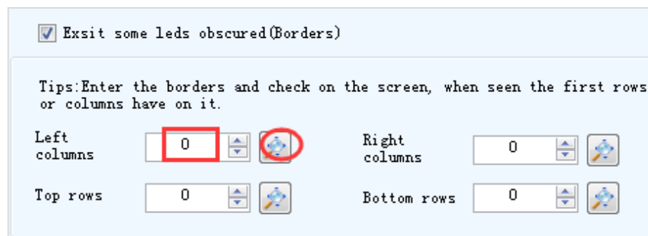
Figure 2-5 Border Settings
