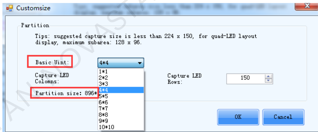
Figure 2-4 Custom Partition
